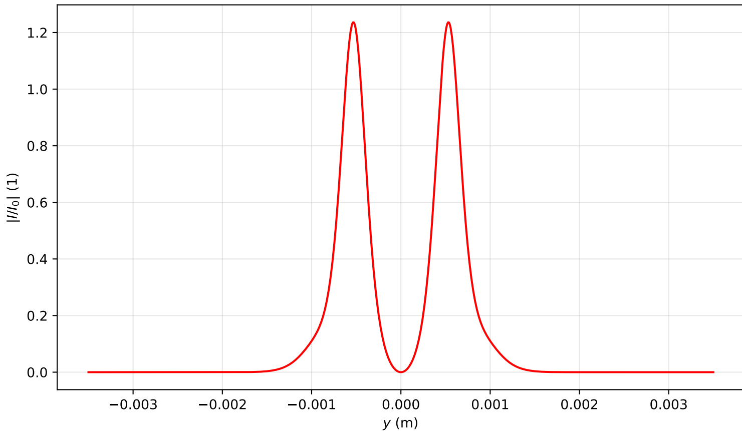
Intensity profile I(x = 0, y, z = 0.557)/I_0 , P_{in}=6.0P_{cr} , artificial time
